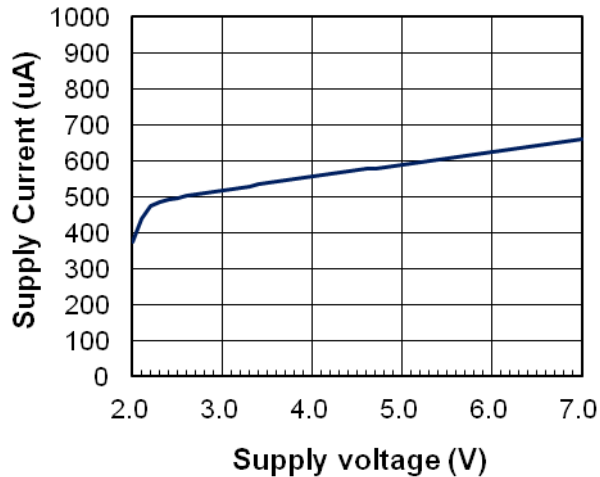
[ Fig.4 ] Supply Current vs. Voltage
