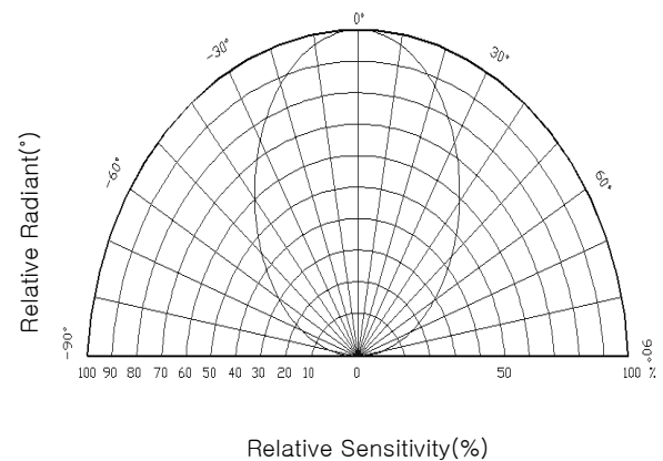
[ Fig.7 ] Directivity
