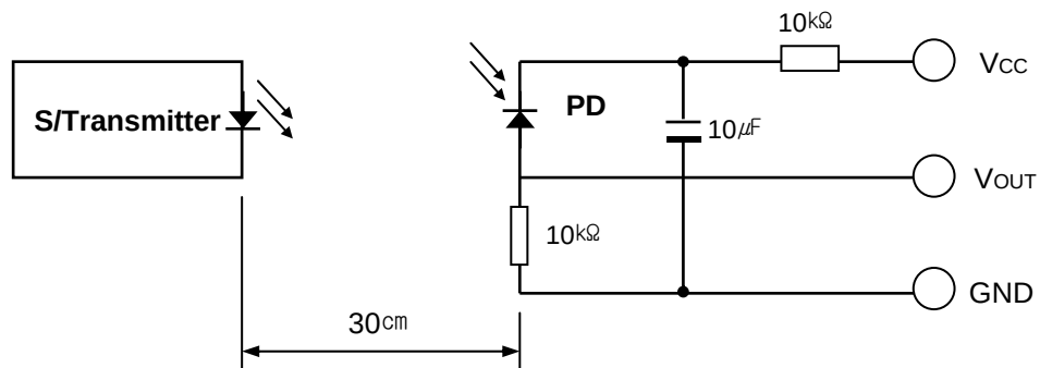
[ Fig.2 ] Transmitter
