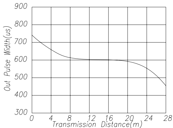
[ Fig.6 ] Output Pulse Width vs. Distance
