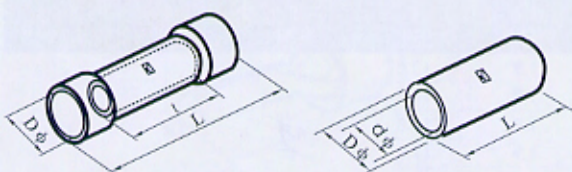
INSULATED BUTT CONNECTORS
