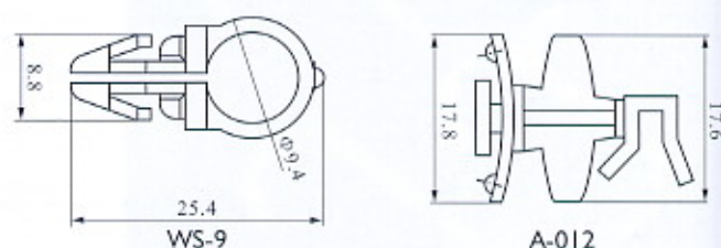
圆形夹线套 Wire Saddle
